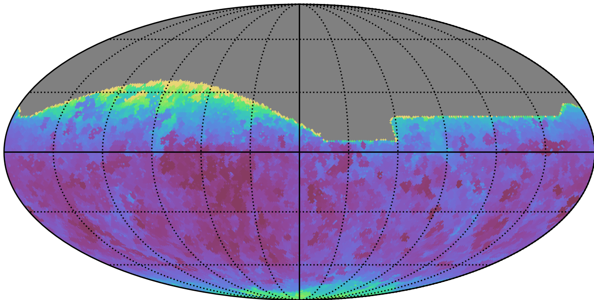
too_10_1v3.4_10yrs All sky all bands: Min seeingEff
