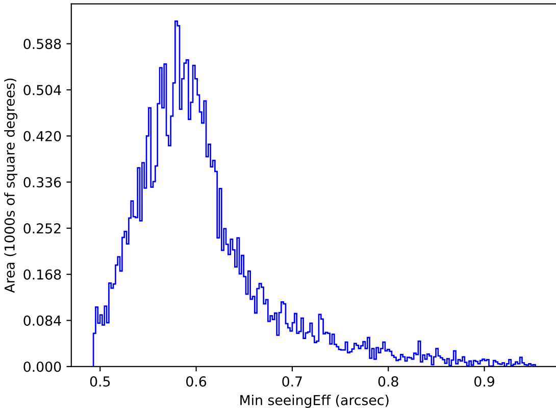
too_10_1v3.4_10yrs All sky all bands: Min seeingEff
