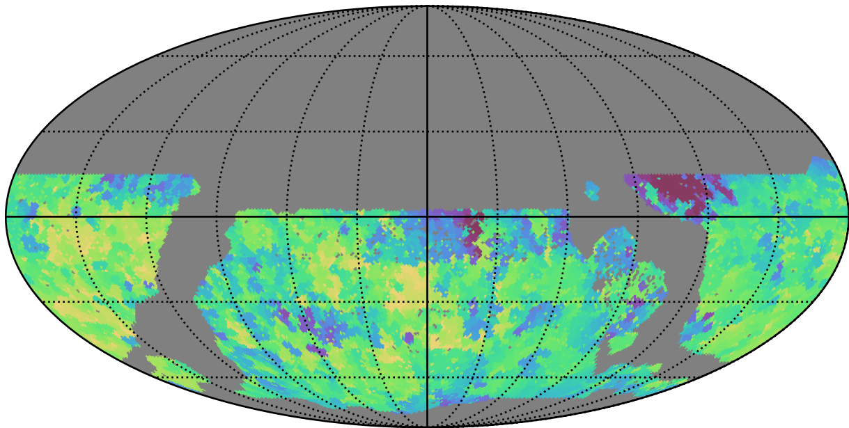
too_10_1v3.4_10yrs WFD u band: Min saturation_mag
