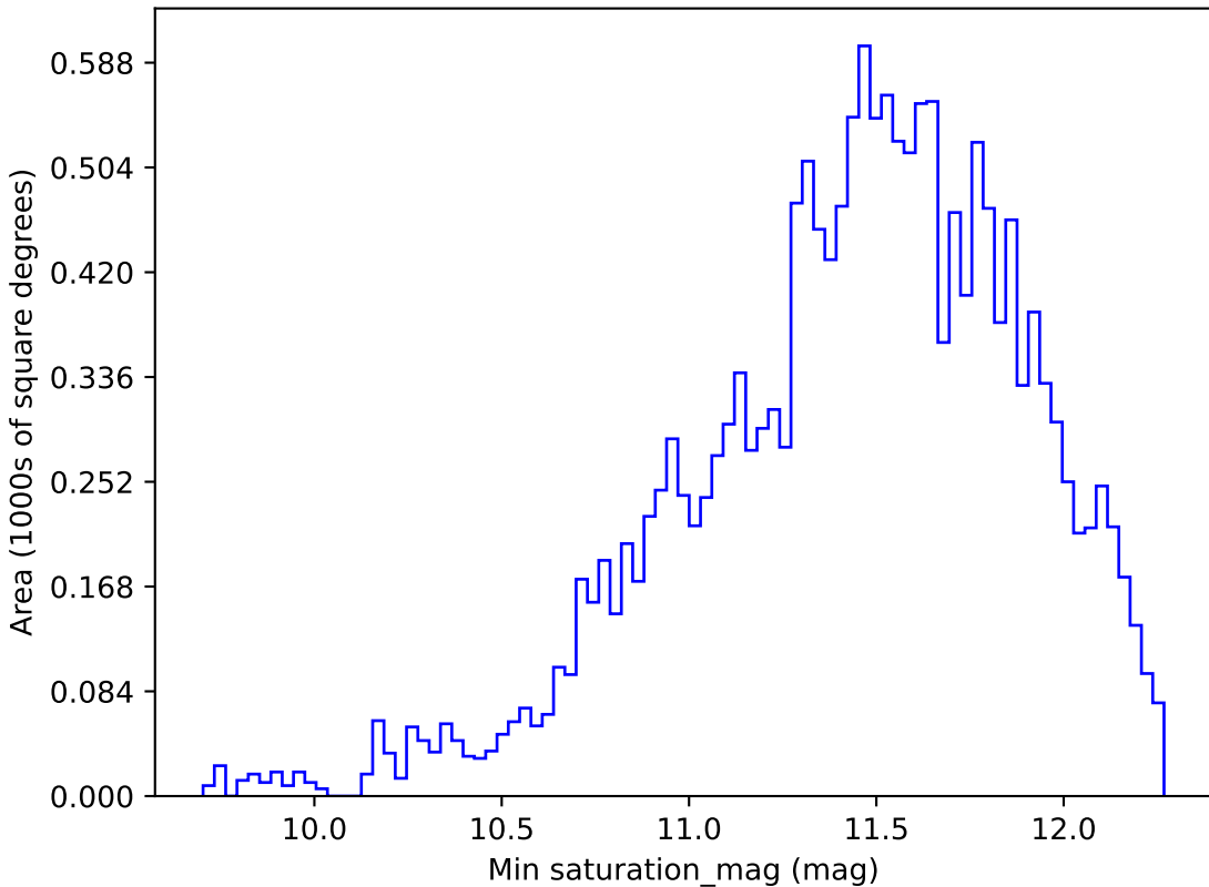
too_10_1v3.4_10yrs WFD u band: Min saturation_mag
