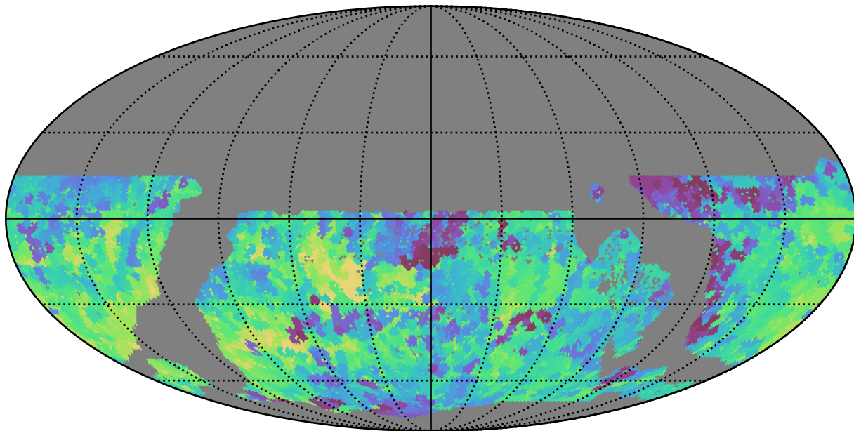
too_10_1v3.4_10yrs WFD r band: Min saturation_mag
