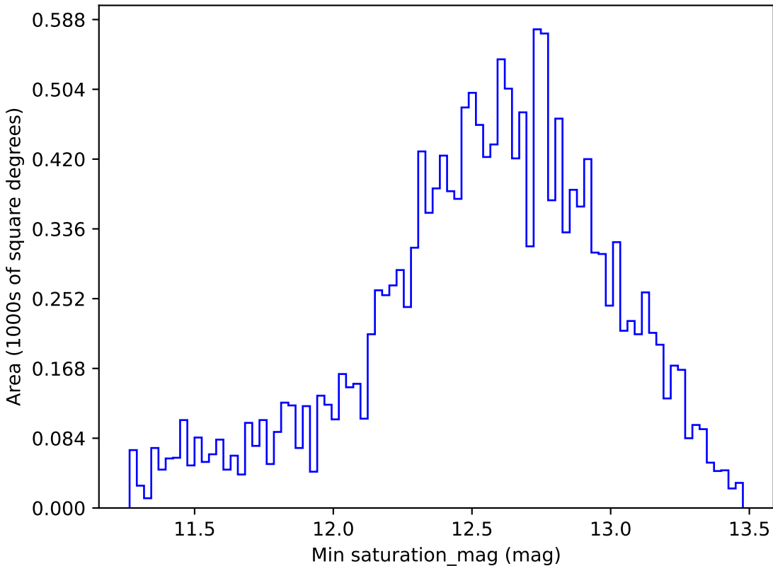
too_10_1v3.4_10yrs WFD r band: Min saturation_mag
