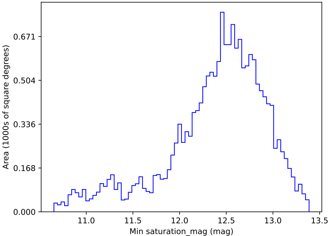
too_10_1v3.4_10yrs WFD i band: Min saturation_mag
