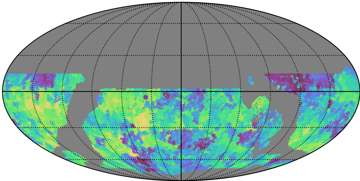
too_10_1v3.4_10yrs WFD g band: Min saturation_mag
