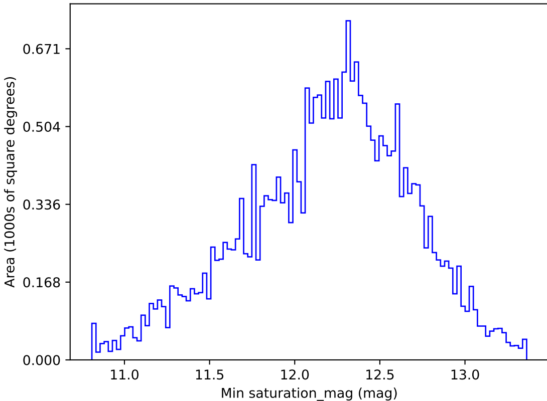
too_10_1v3.4_10yrs All sky z band: Min saturation_mag
