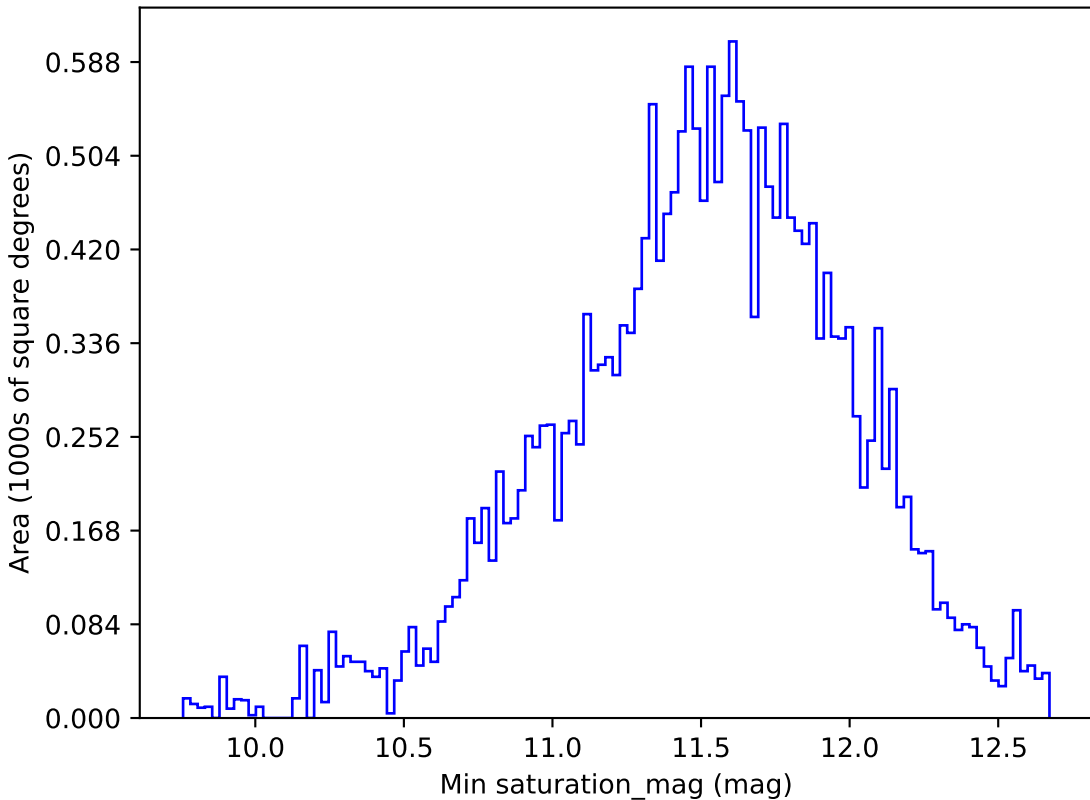
too_10_1v3.4_10yrs All sky u band: Min saturation_mag
