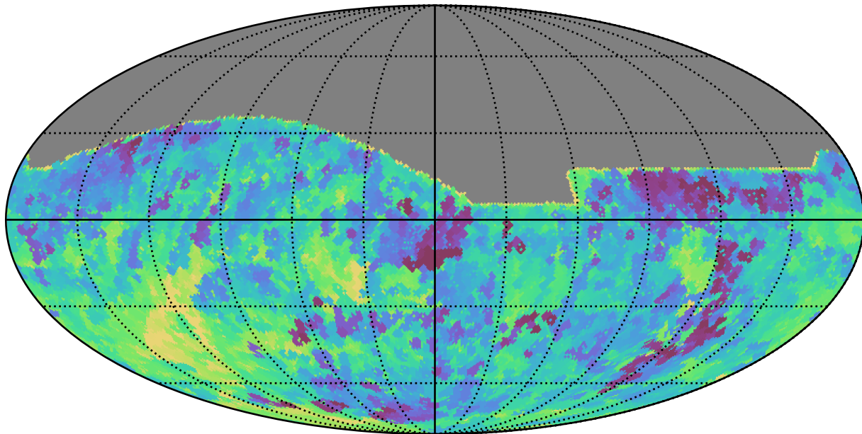
too_10_1v3.4_10yrs All sky r band: Min saturation_mag
