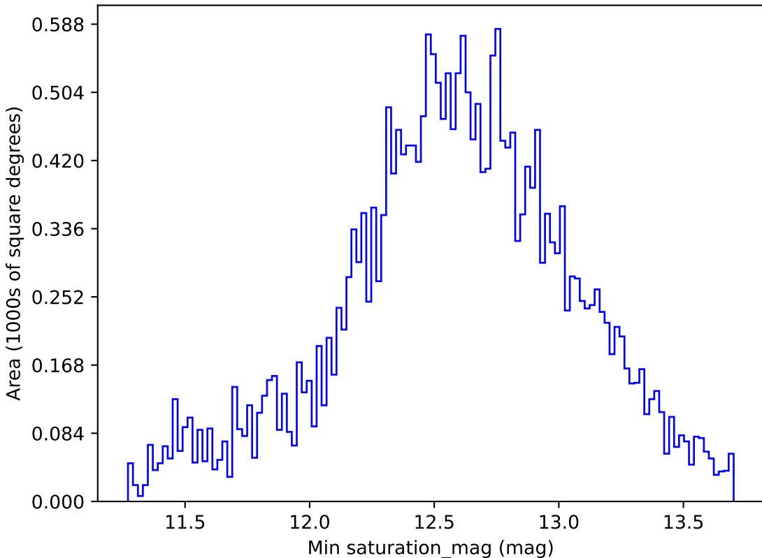
too_10_1v3.4_10yrs All sky r band: Min saturation_mag
