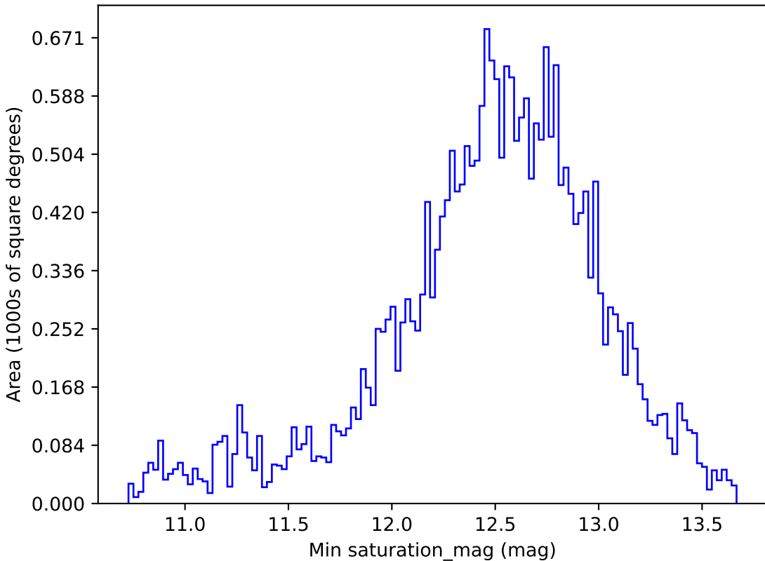
too_10_1v3.4_10yrs All sky i band: Min saturation_mag
