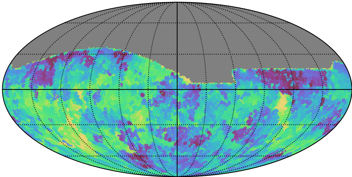
too_10_1v3.4_10yrs All sky g band: Min saturation_mag
