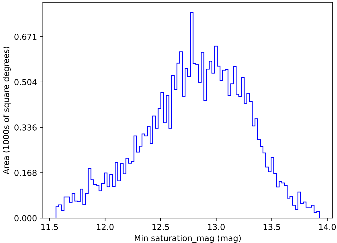
too_10_1v3.4_10yrs All sky g band: Min saturation_mag
