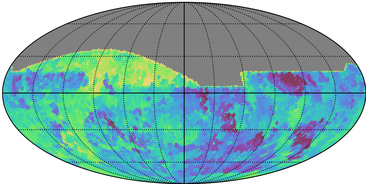
too_10_1v3.4_10yrs All sky all bands: Min saturation_mag
