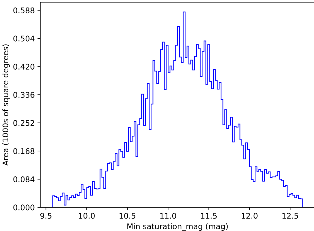
too_10_1v3.4_10yrs All sky all bands: Min saturation_mag
