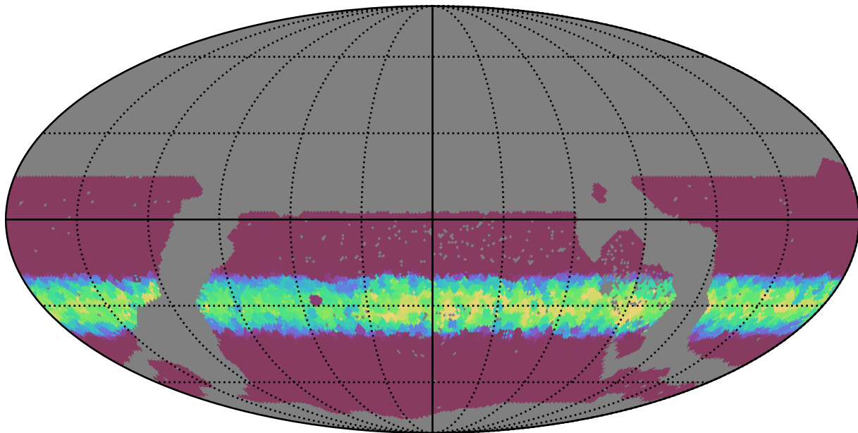
too_10_1v3.4_10yrs WFD z band: Min normairmass
