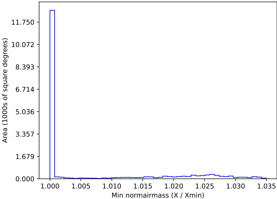
too_10_1v3.4_10yrs WFD z band: Min normairmass
