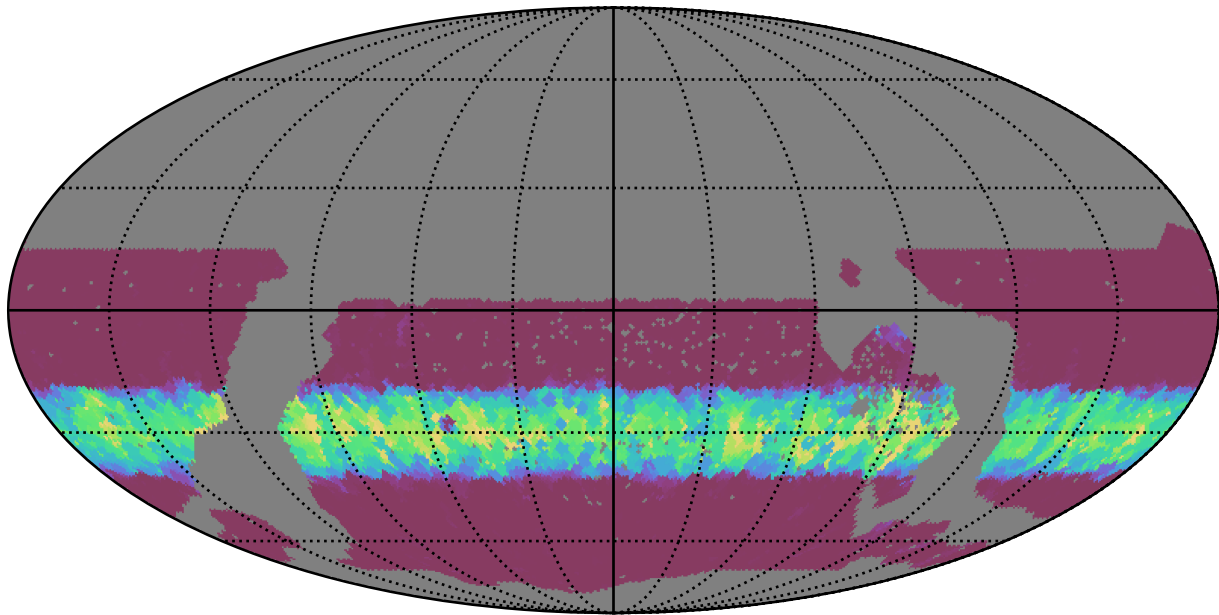
too_10_1v3.4_10yrs WFD u band: Min normairmass
