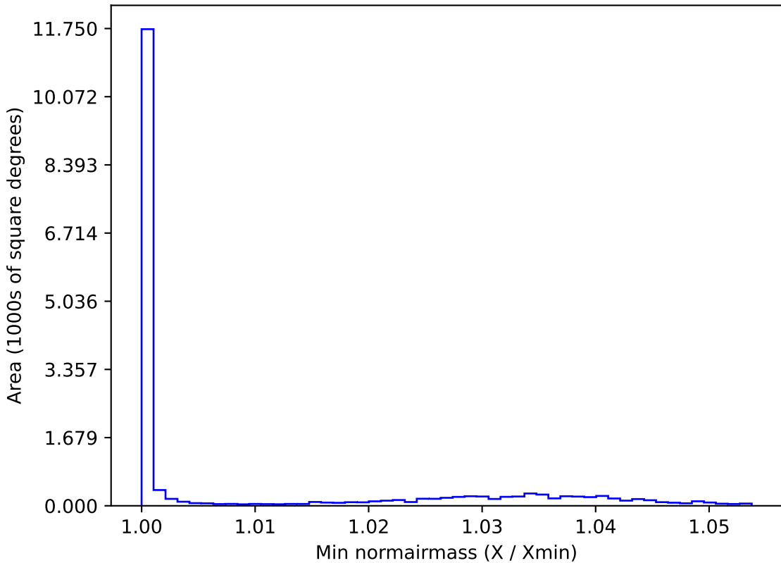
too_10_1v3.4_10yrs WFD u band: Min normairmass
