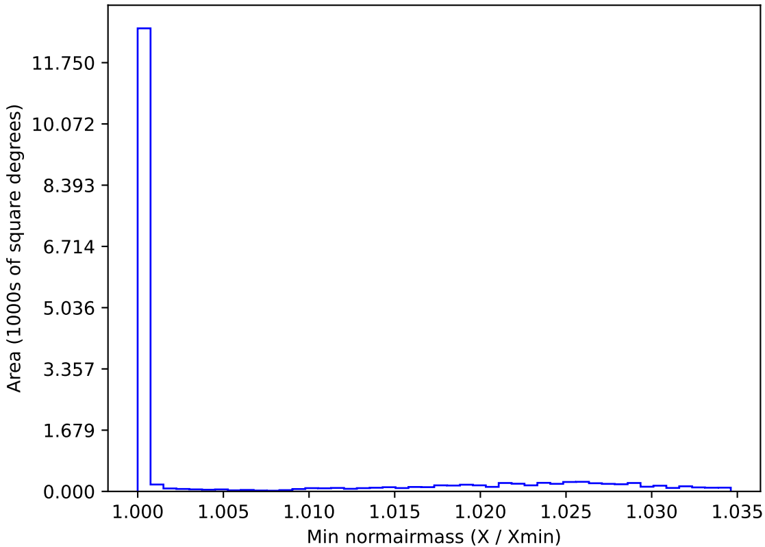
too_10_1v3.4_10yrs WFD i band: Min normairmass
