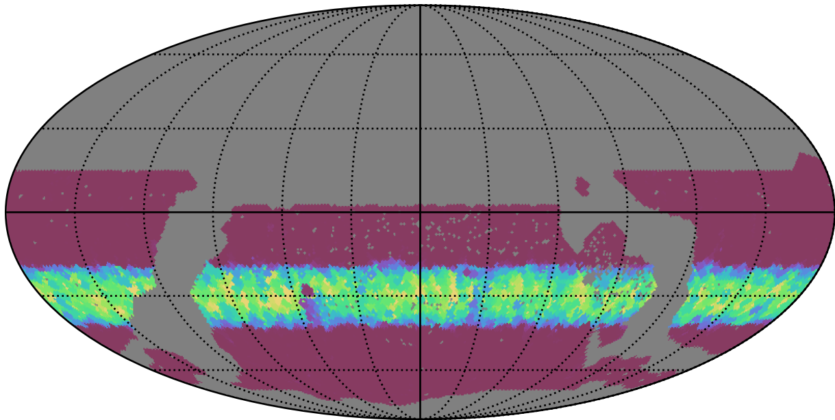
too_10_1v3.4_10yrs WFD g band: Min normairmass
