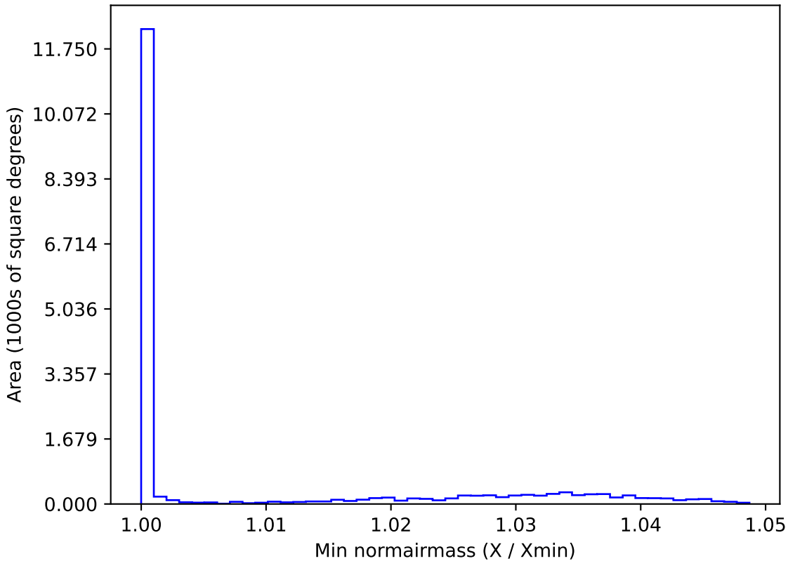
too_10_1v3.4_10yrs WFD g band: Min normairmass
