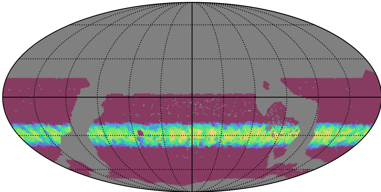
too_10_1v3.4_10yrs WFD all bands: Min normairmass
