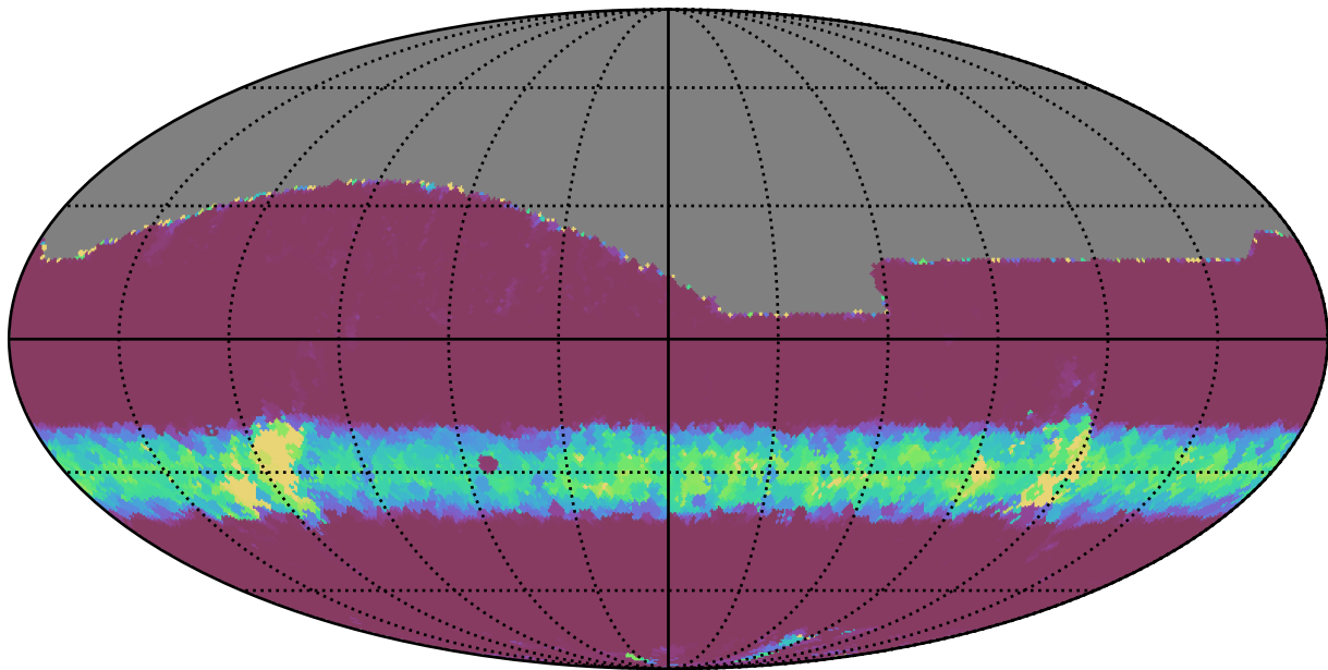
too_10_1v3.4_10yrs All sky z band: Min normairmass
