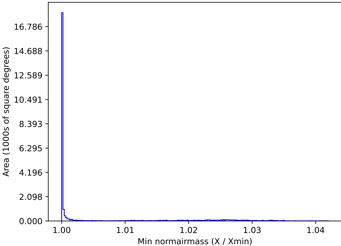
too_10_1v3.4_10yrs All sky z band: Min normairmass
