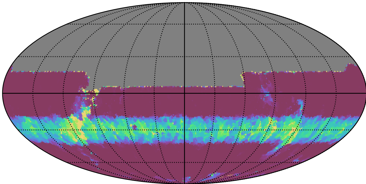
too_10_1v3.4_10yrs All sky u band: Min normairmass
