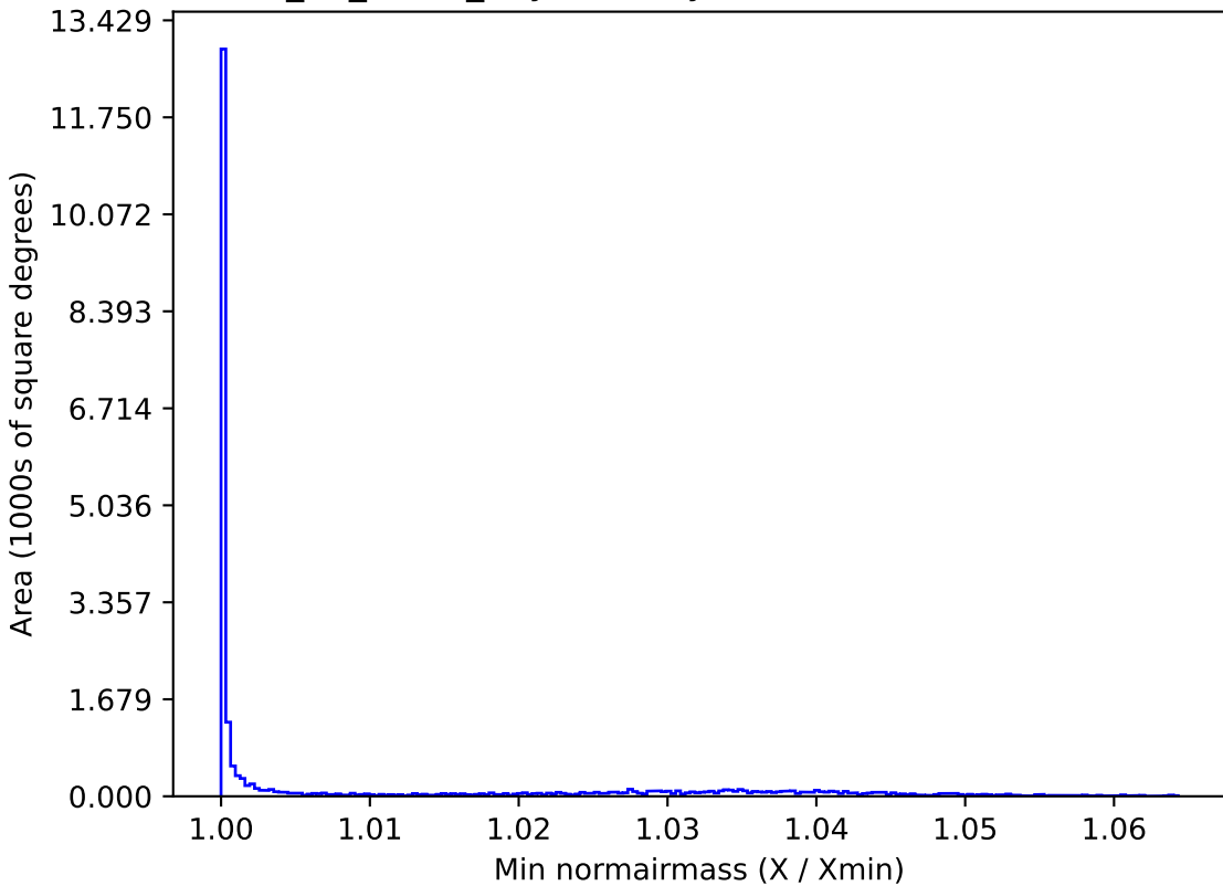
too_10_1v3.4_10yrs All sky u band: Min normairmass
