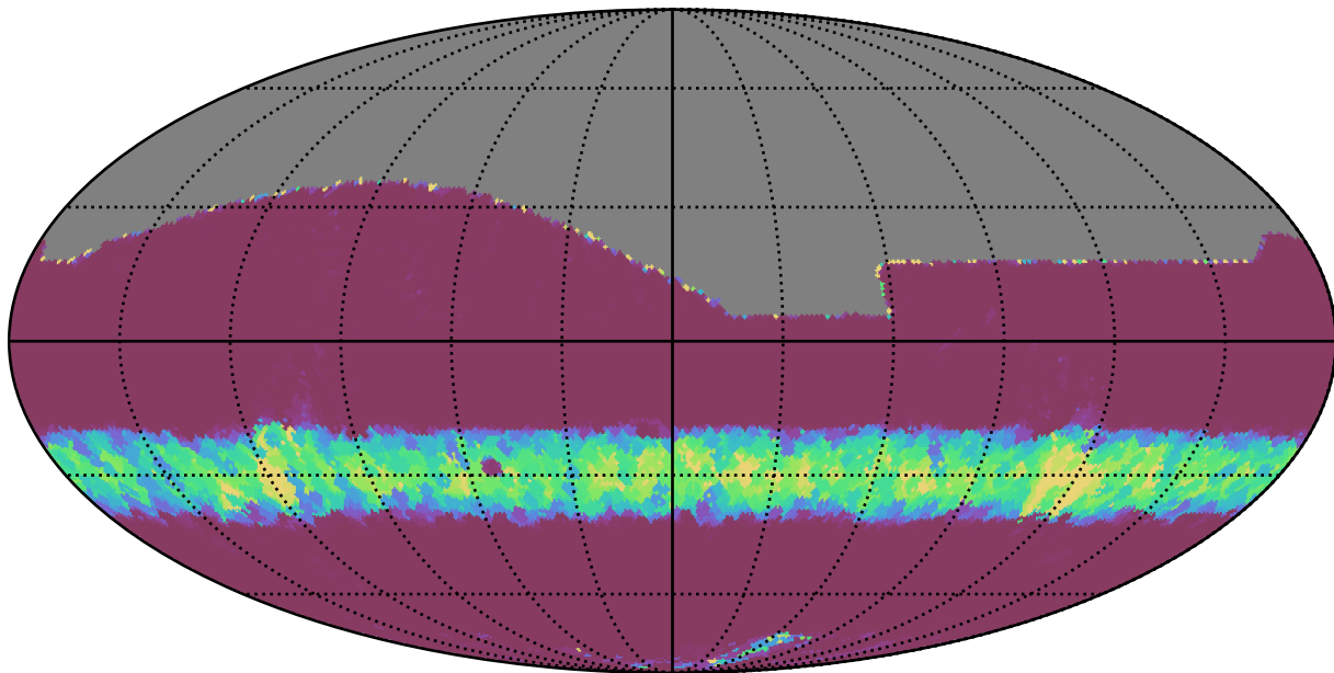
too_10_1v3.4_10yrs All sky r band: Min normairmass
