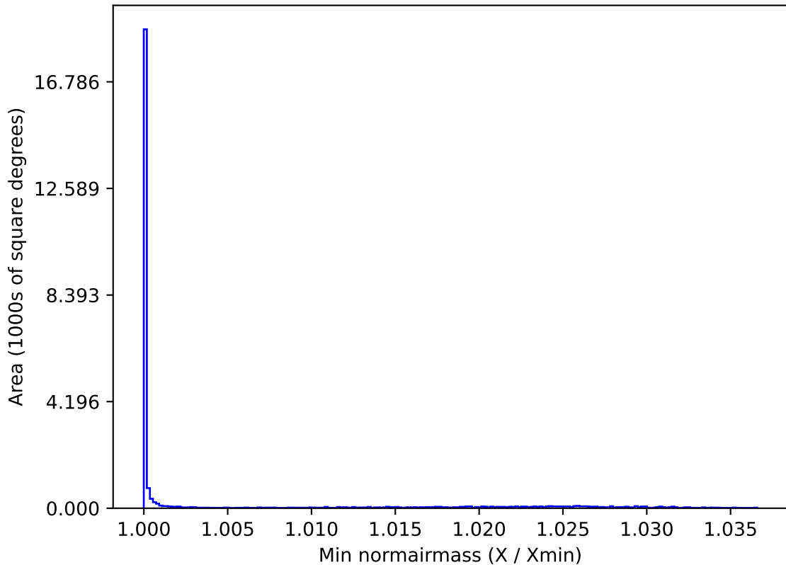
too_10_1v3.4_10yrs All sky r band: Min normairmass
