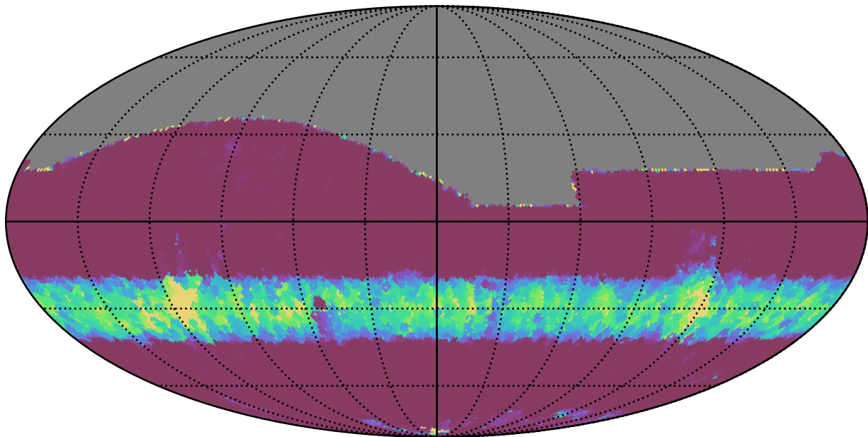
too_10_1v3.4_10yrs All sky g band: Min normairmass
