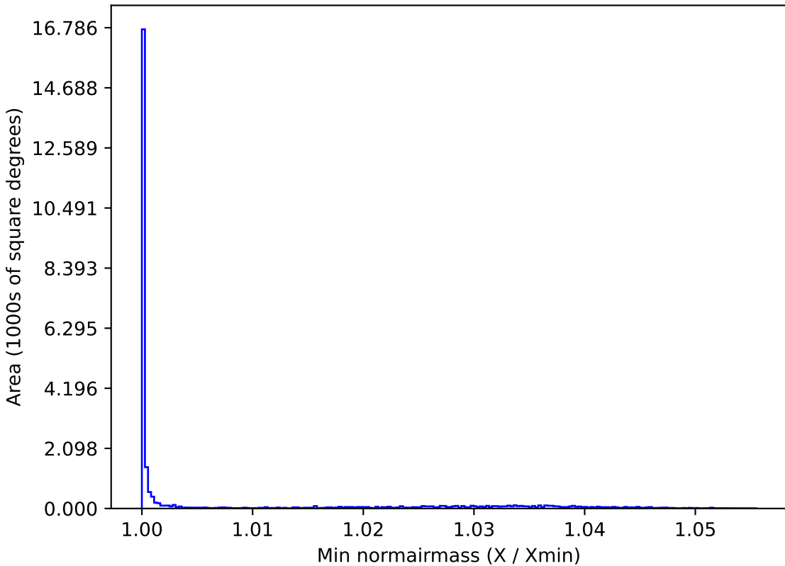
too_10_1v3.4_10yrs All sky g band: Min normairmass
