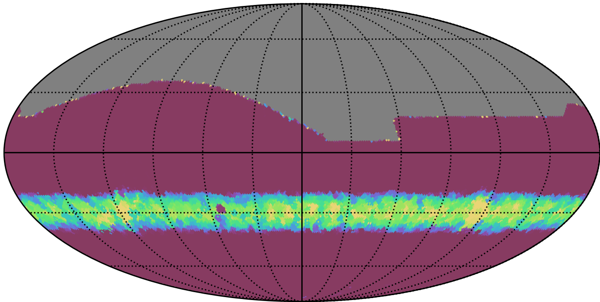
too_10_1v3.4_10yrs All sky all bands: Min normairmass
