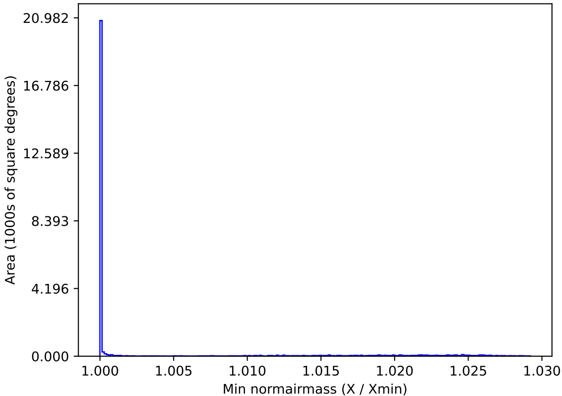
too_10_1v3.4_10yrs All sky all bands: Min normairmass
