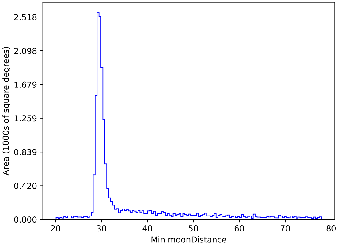
too_10_1v3.4_10yrs WFD z band: Min moonDistance
