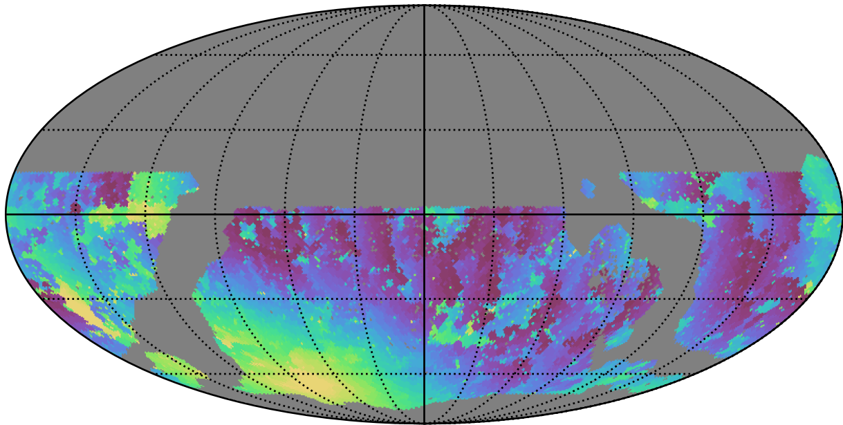
too_10_1v3.4_10yrs WFD u band: Min moonDistance
