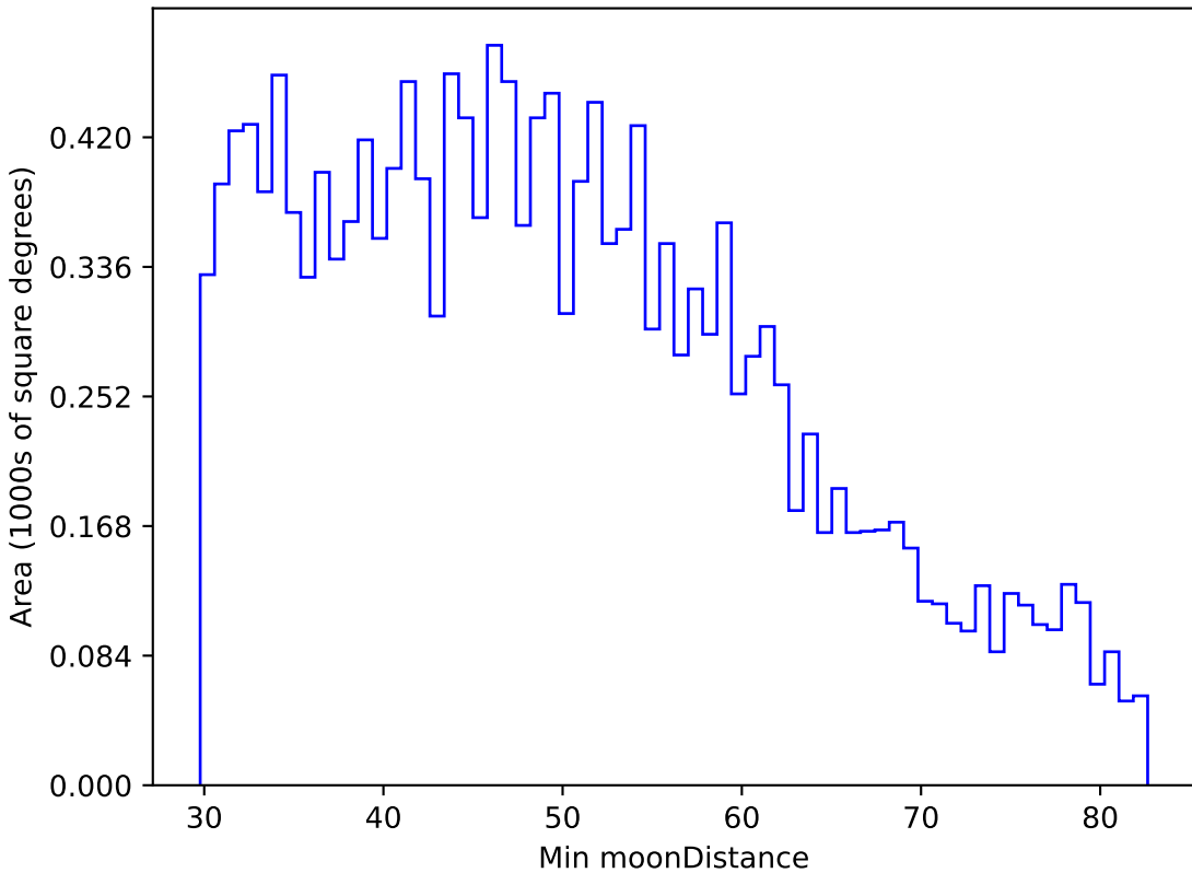
too_10_1v3.4_10yrs WFD u band: Min moonDistance
