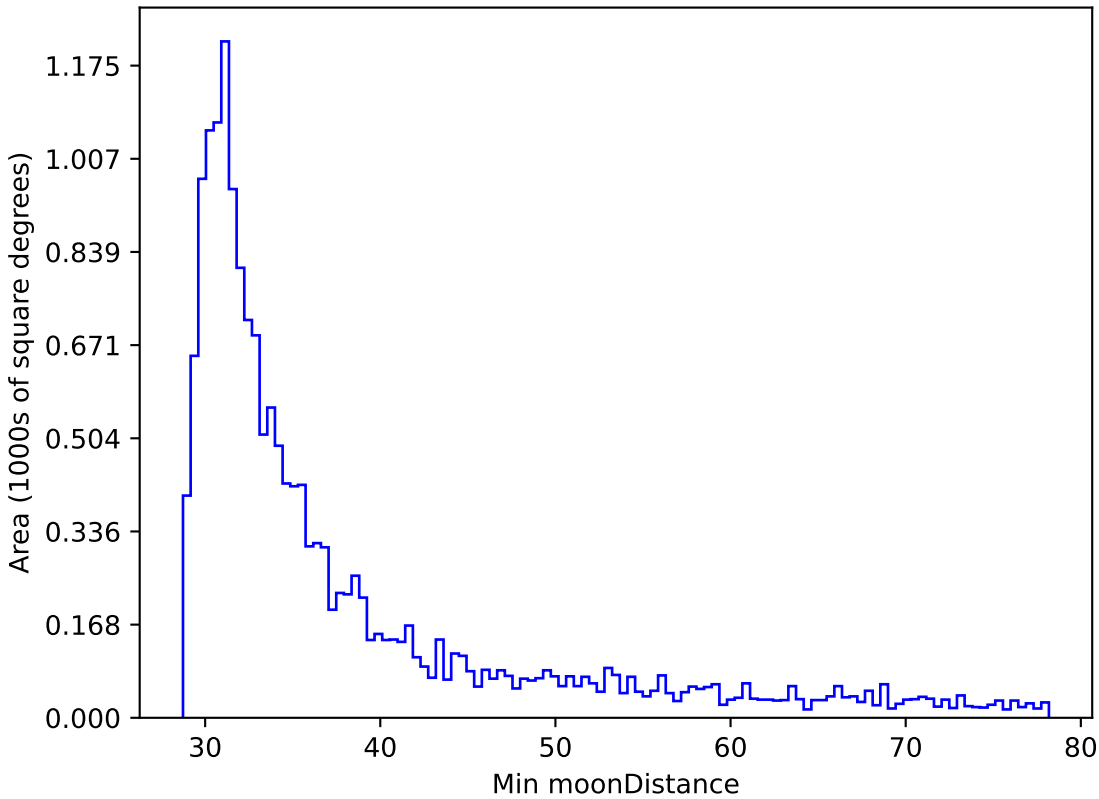
too_10_1v3.4_10yrs WFD r band: Min moonDistance
