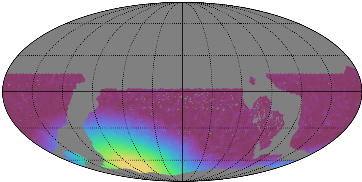
too_10_1v3.4_10yrs WFD i band: Min moonDistance
