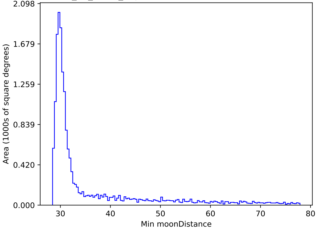
too_10_1v3.4_10yrs WFD i band: Min moonDistance
