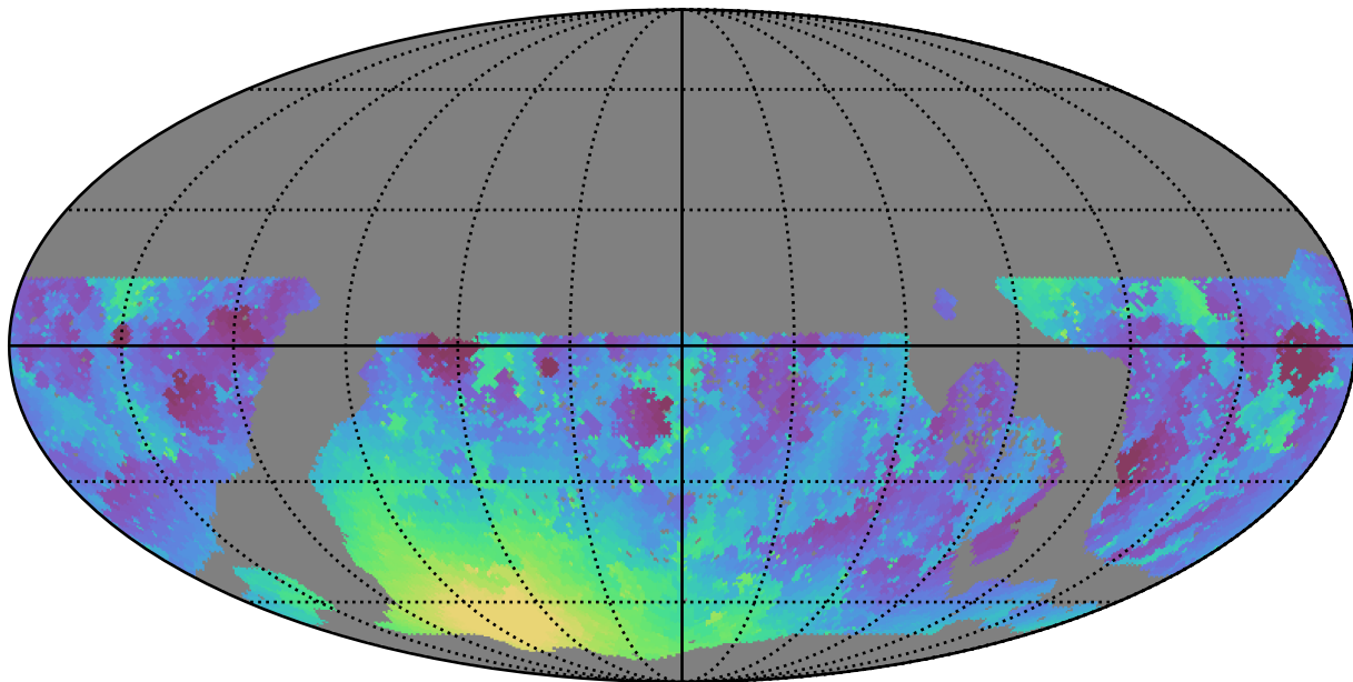
too_10_1v3.4_10yrs WFD g band: Min moonDistance
