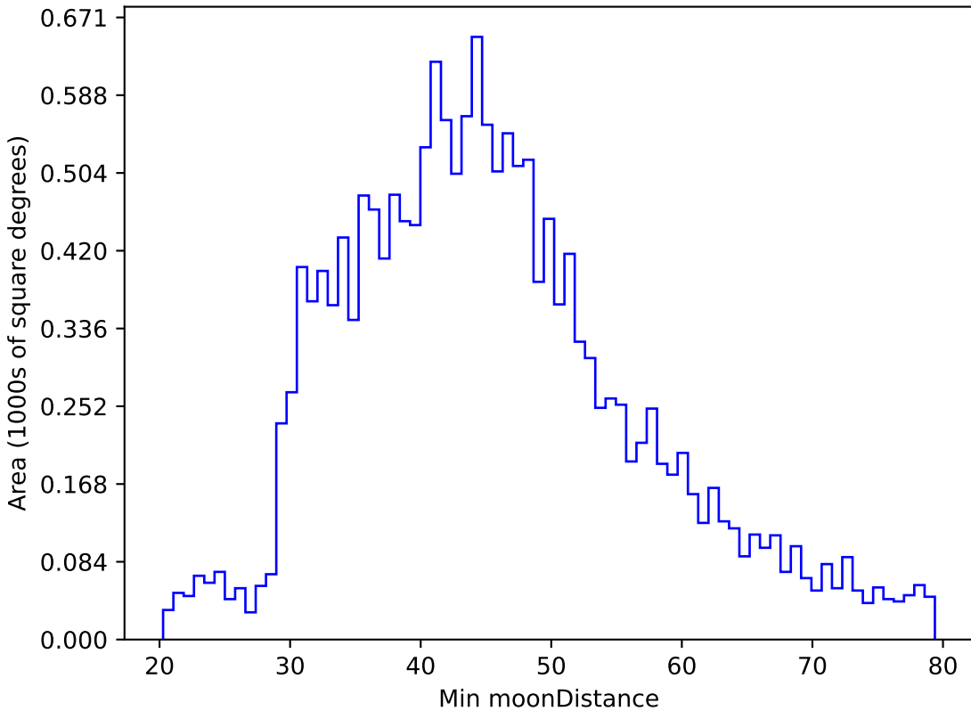
too_10_1v3.4_10yrs WFD g band: Min moonDistance
