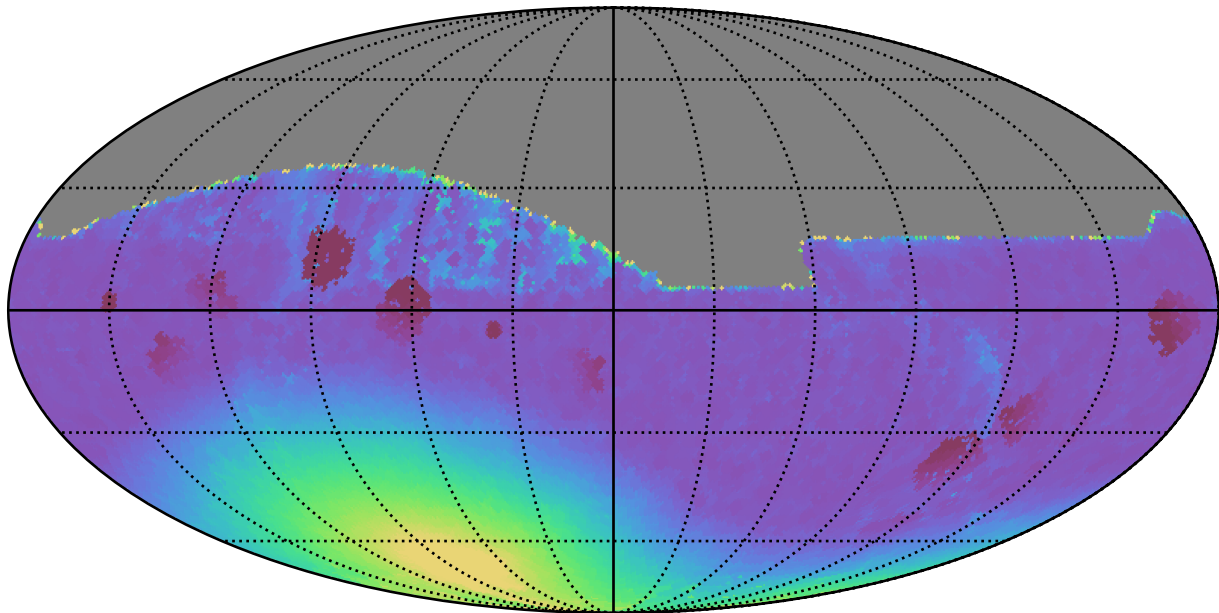
too_10_1v3.4_10yrs All sky z band: Min moonDistance
