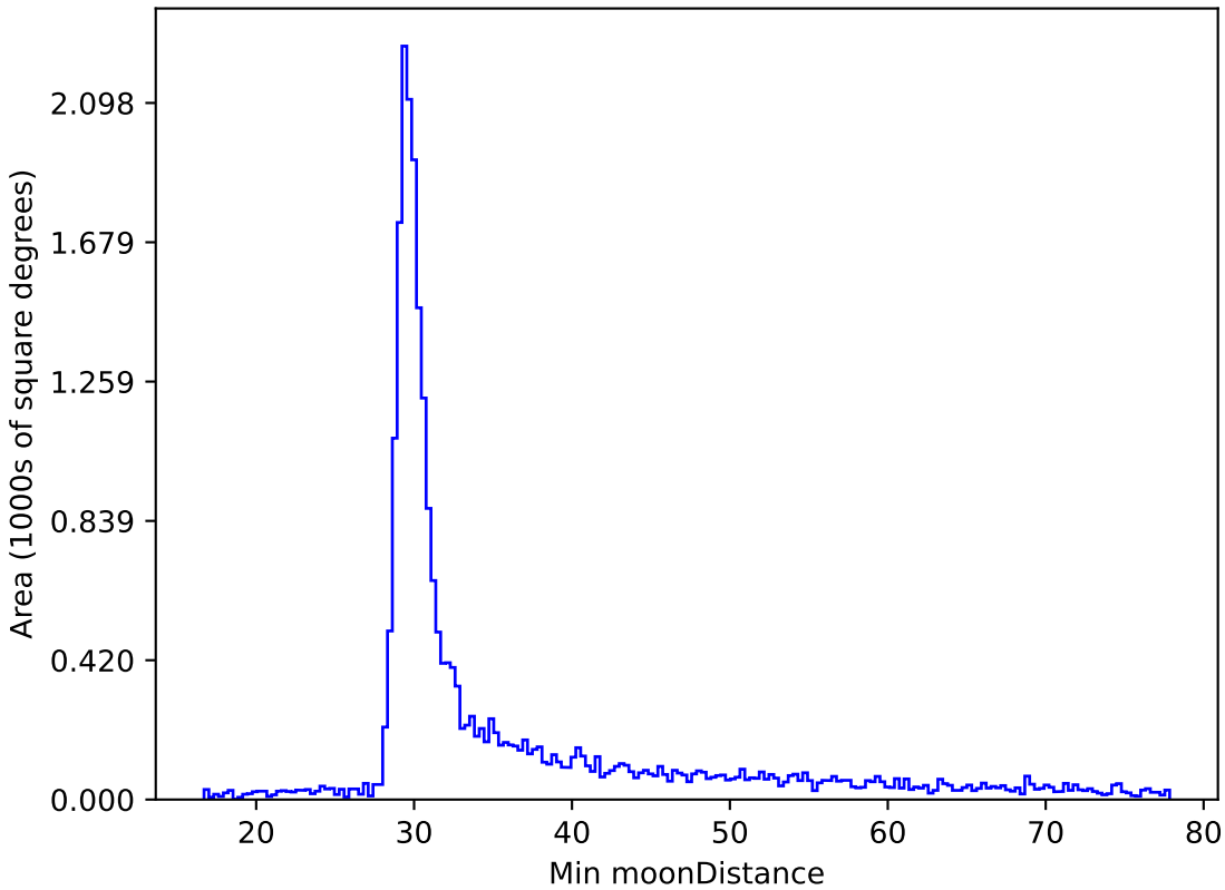
too_10_1v3.4_10yrs All sky z band: Min moonDistance
