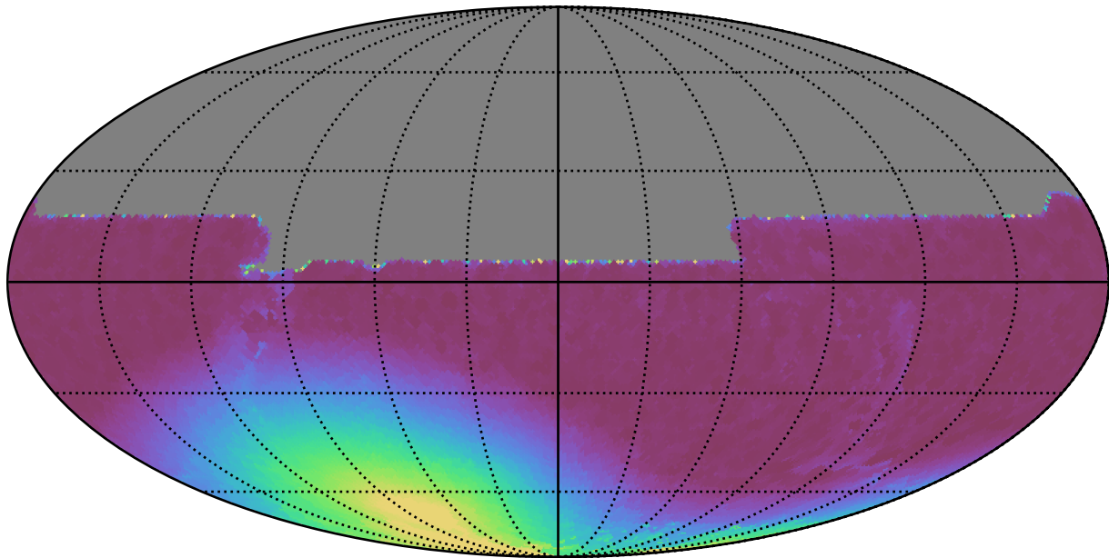
too_10_1v3.4_10yrs All sky y band: Min moonDistance
