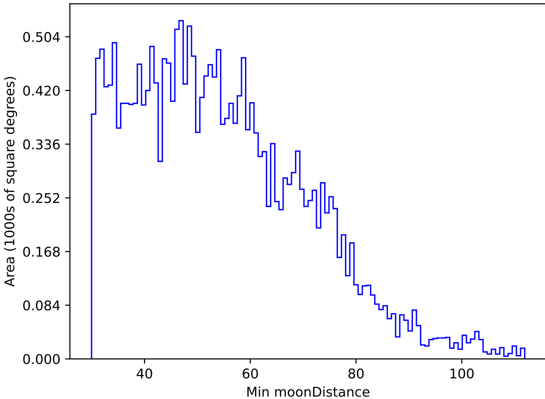
too_10_1v3.4_10yrs All sky u band: Min moonDistance
