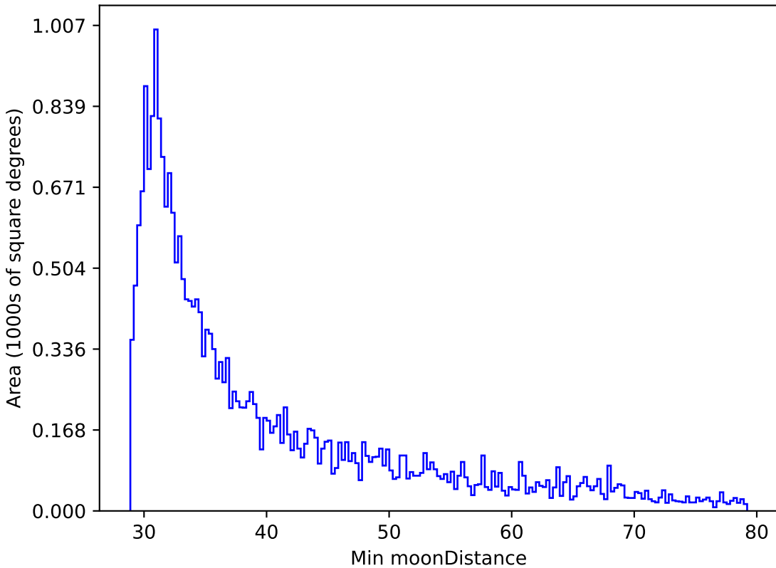
too_10_1v3.4_10yrs All sky r band: Min moonDistance
