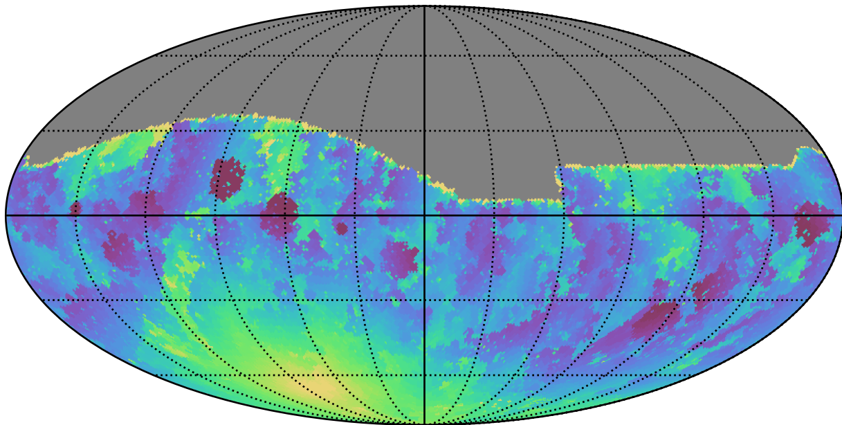
too_10_1v3.4_10yrs All sky g band: Min moonDistance
