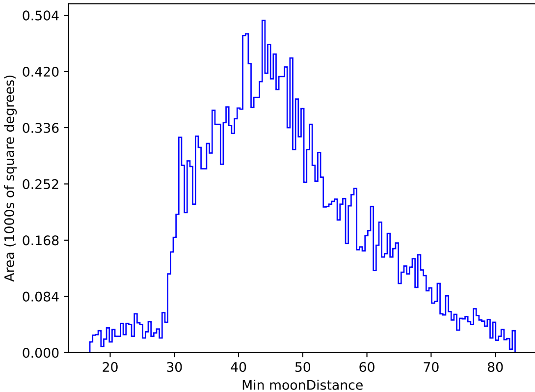
too_10_1v3.4_10yrs All sky g band: Min moonDistance
